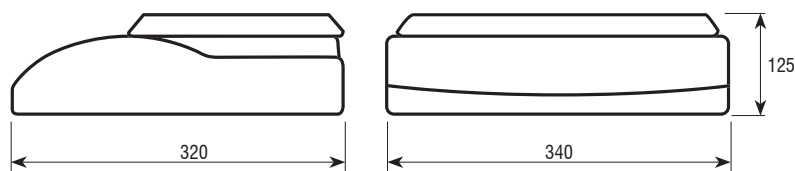
Dimensions (mm)
